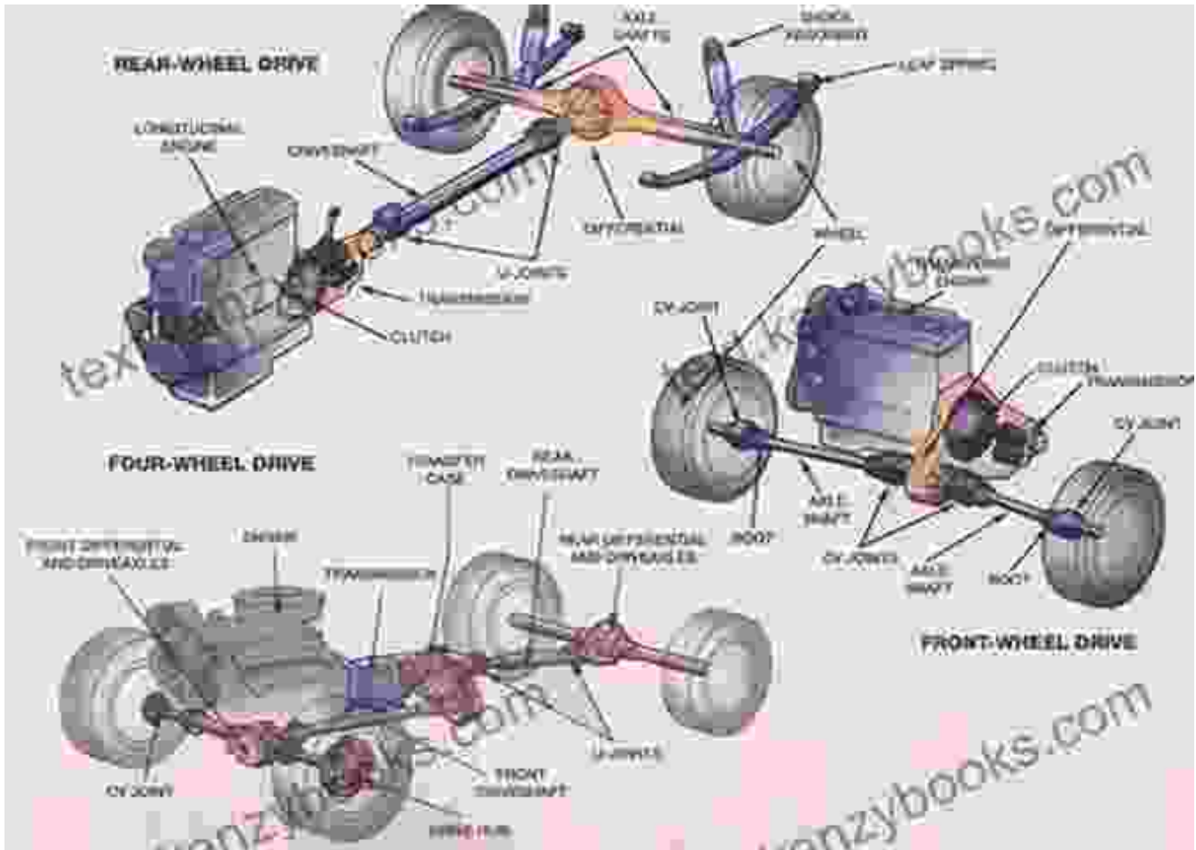
Off-Road Vehicle Drivetrain
